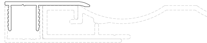
FINISH BOARD BASE + INTERLOCKING BOARD EXAMPLE + FINISH BOARD CAP (40MM) - ASSEMBLED
