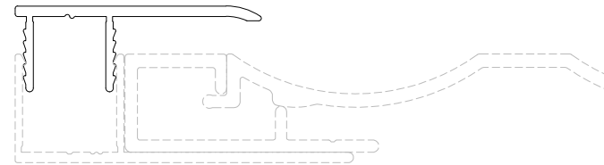
FINISH BOARD BASE + INTERLOCKING BOARD EXAMPLE + FINISH BOARD CAP (40MM) - ASSEMBLY
