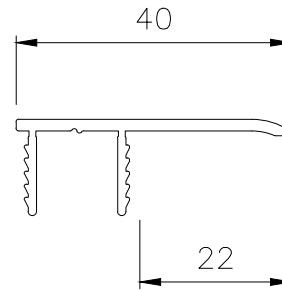
40MM CLADDING FINISH BOARD CAP (TEX8160)
